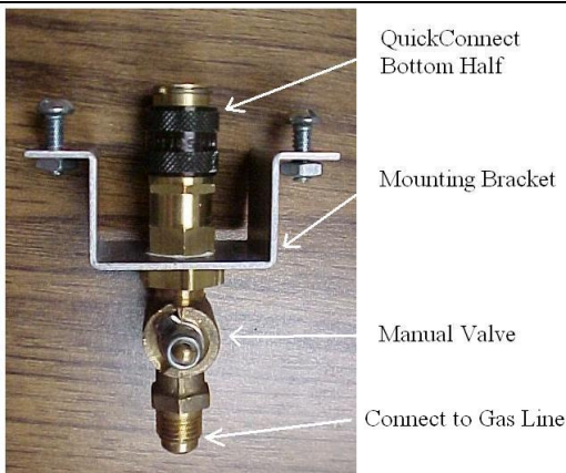
Gas line connection with optional QuickConnect fitting and mounting bracket.
